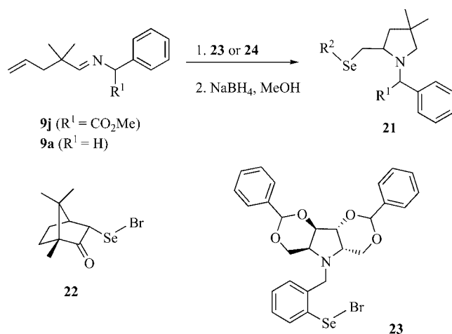
Scheme 5. Cyclisation of N -(alkenylidene)alkylamines 9 with chiral selenyl bromides.
