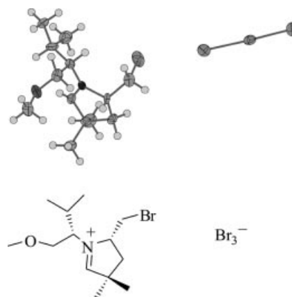
Figure 1. X-ray crystal analysis of the tribromide of the 5 S stereoisomer of 10e .
