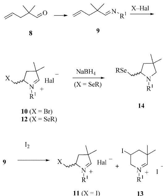
Scheme 2. Cyclisation of optically active N -(alkenylidene)alkylamines (chiral \text{R}^1 ) with achiral electrophiles.
