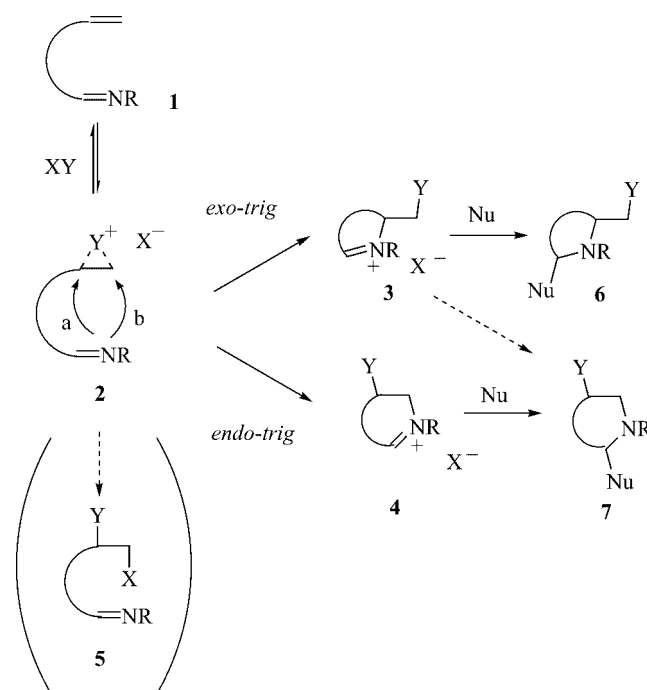
Scheme 1. General mechanism of the electrophile-induced cyclisation of unsaturated imines.
