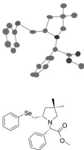
Figure 2. X-ray crystal analysis of the 5 S stereoisomer of the pyrrolidine 14f (major isomer).
