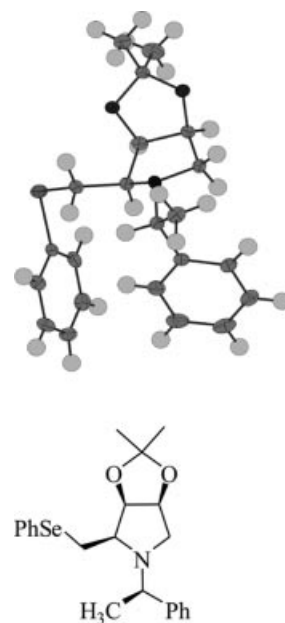
Figure 3. X-ray crystal analysis of the 5 S stereoisomer of 20d .
