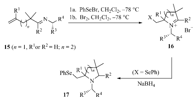
Scheme 3. Cyclisation of optically active N -(alkenylidene)alkylamines 15 .
